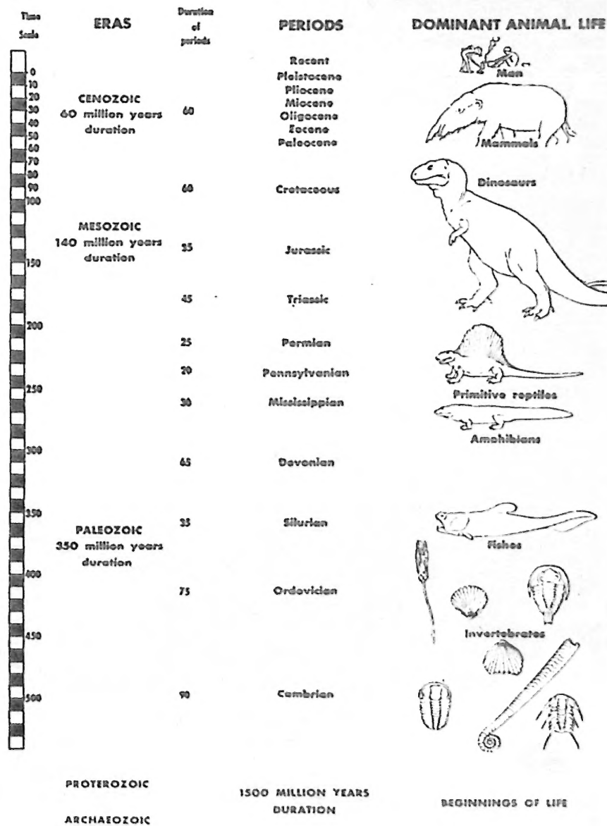
Figure 2. Geological time chart. After Colbert. Courtesy American Museum of Natural History. (Neg. J9958)
